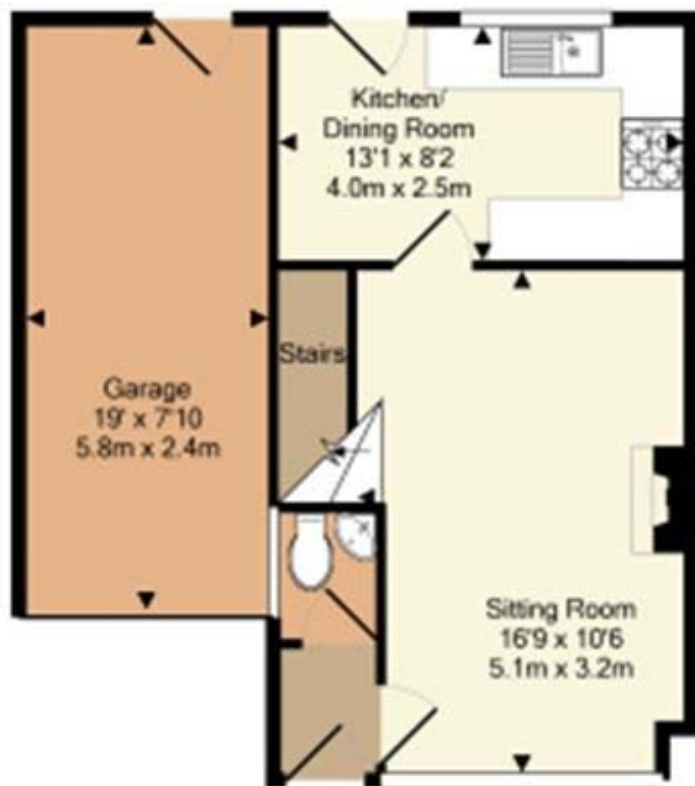
Ground Floor Approx. Floor Area 473 Sq.Ft. (43.9 Sq.M.)
